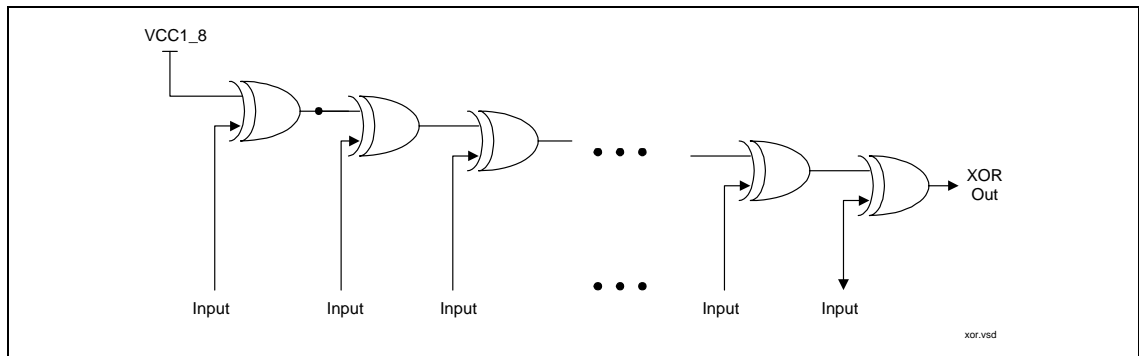
Figure 10. XOR-Tree Chain
