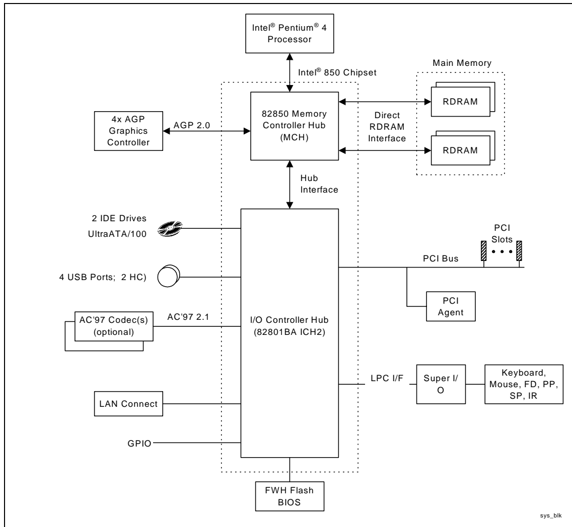
Figure 1. Intel® 82850 Desktop System Block Diagram
