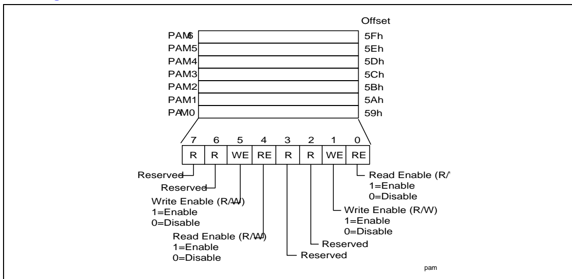
Figure 2. PAM Registers and Attribute Bits
