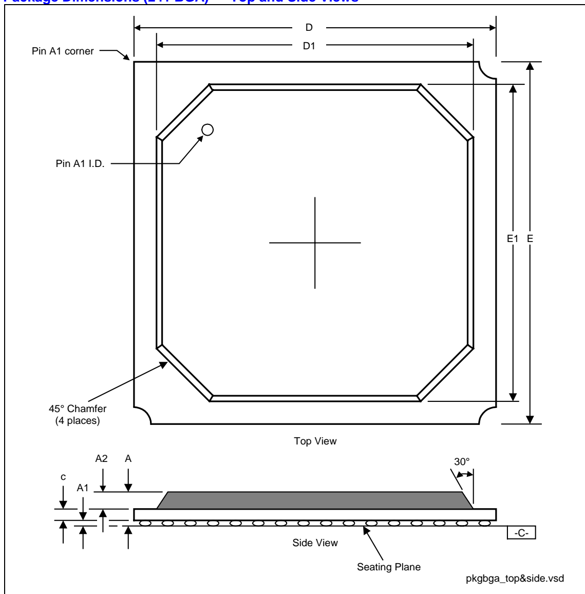
Figure 8. Package Dimensions (241 BGA) — Top and Side Views
